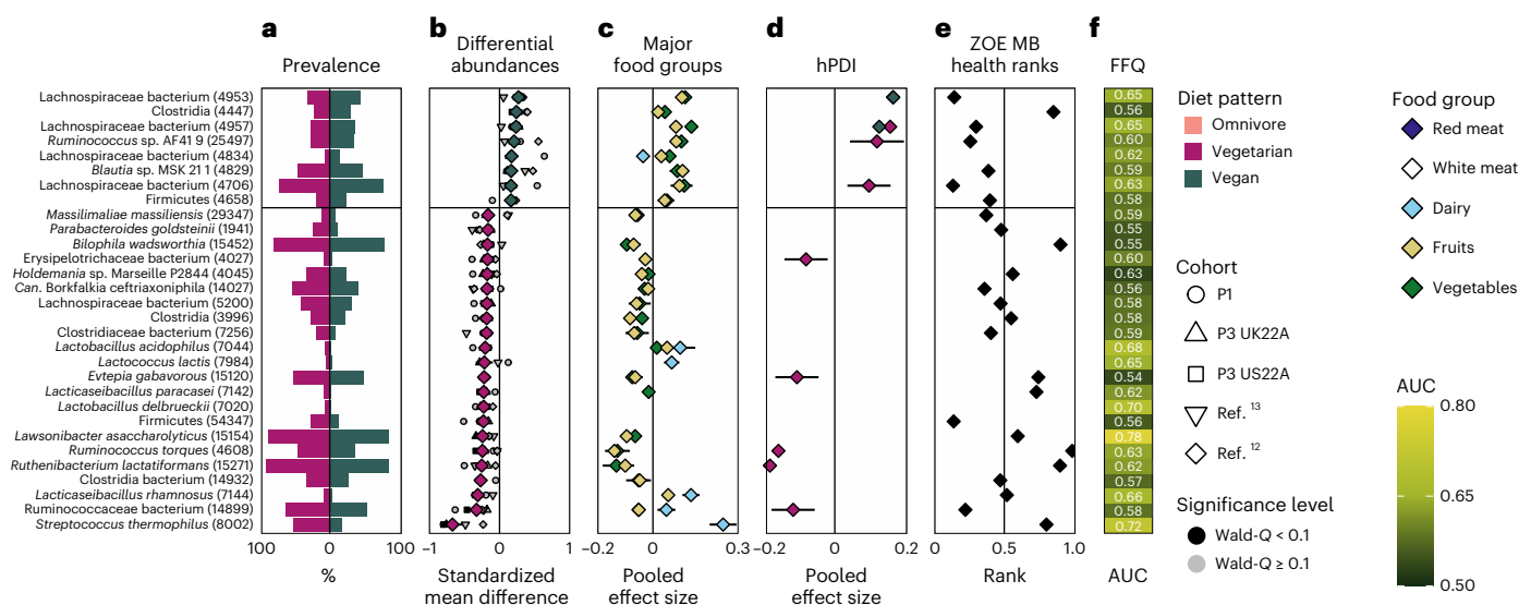
Fig. 4 | Gut microbial signatures of a vegetarian vs vegan diet. a , Prevalence of the top 30 signature SGBs (with their respective SGB IDs in parentheses) in vegetarian (left) and vegan (right) gut microbiomes. b , Meta-analysed correlations between SGB relative abundance and diet pattern ( n_{\text{vegetarian}} = 1,088 in purple vs n_{\text{vegan}} = 656 in green). The top 30 SGBs with the largest absolute SMD are reported. Smaller shapes are per-cohort correlations (black indicates Wald q -value < 0.1 , grey indicates Wald q -value \geq 0.1 ). The black horizontal bar indicates the separation between the correlations with vegetarians vs vegans for ease of visualization only. c , Meta-analysed pooled effect sizes with upper and lower confidence intervals from correlations between SGB relative abundance and consumption of five major food groups (meat: n_{\text{P1}} = 841 individuals,
